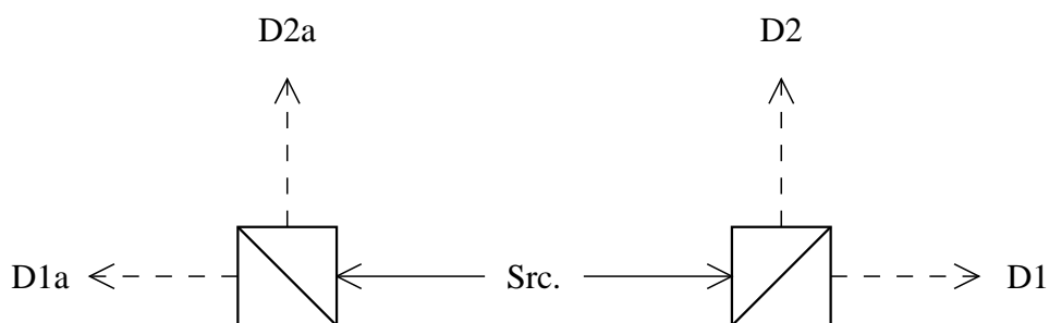
Figure 5: An EPR-type setup
