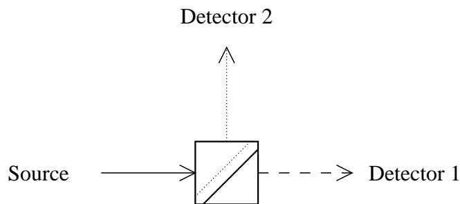
Figure 4: Superpositions of intrinsic states
