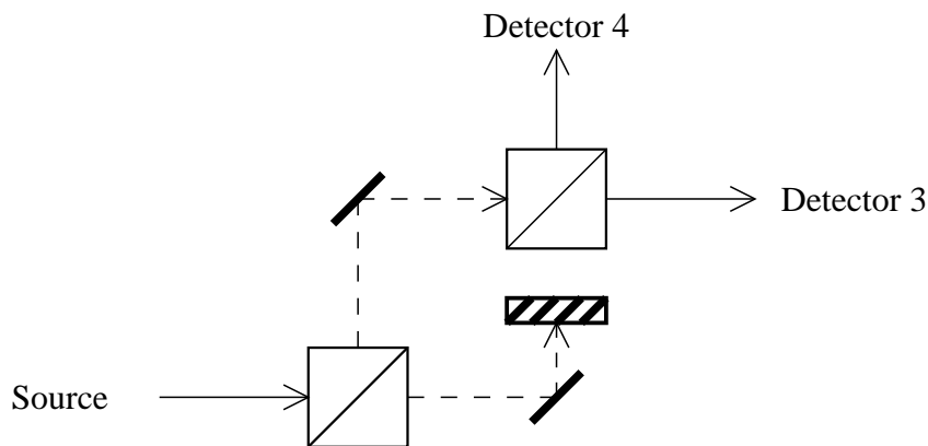
Figure 3: No interference effect with one path blocked
