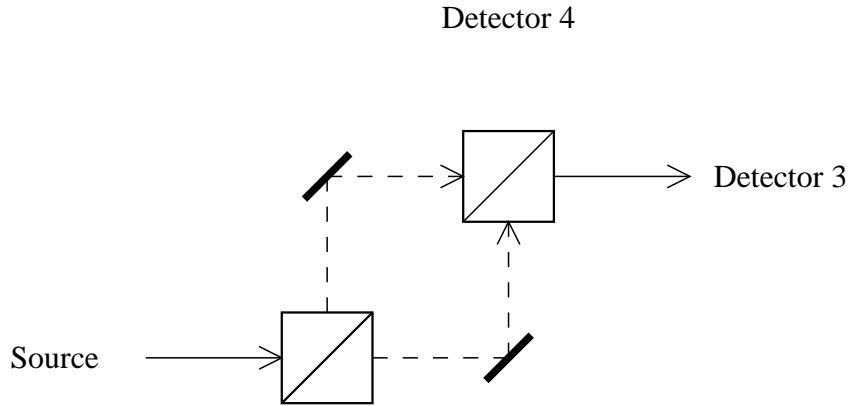
Figure 2: Single particle interference
