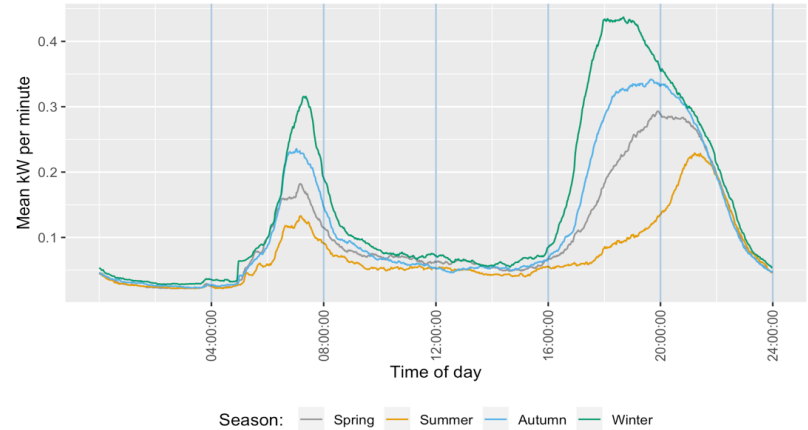
Lighting: seasonal mean power demand profiles
