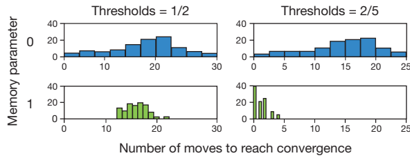
Figure 6: Histograms of number of moves to reach convergence, by memory and acceptability threshold \tau (memory span = 5).
