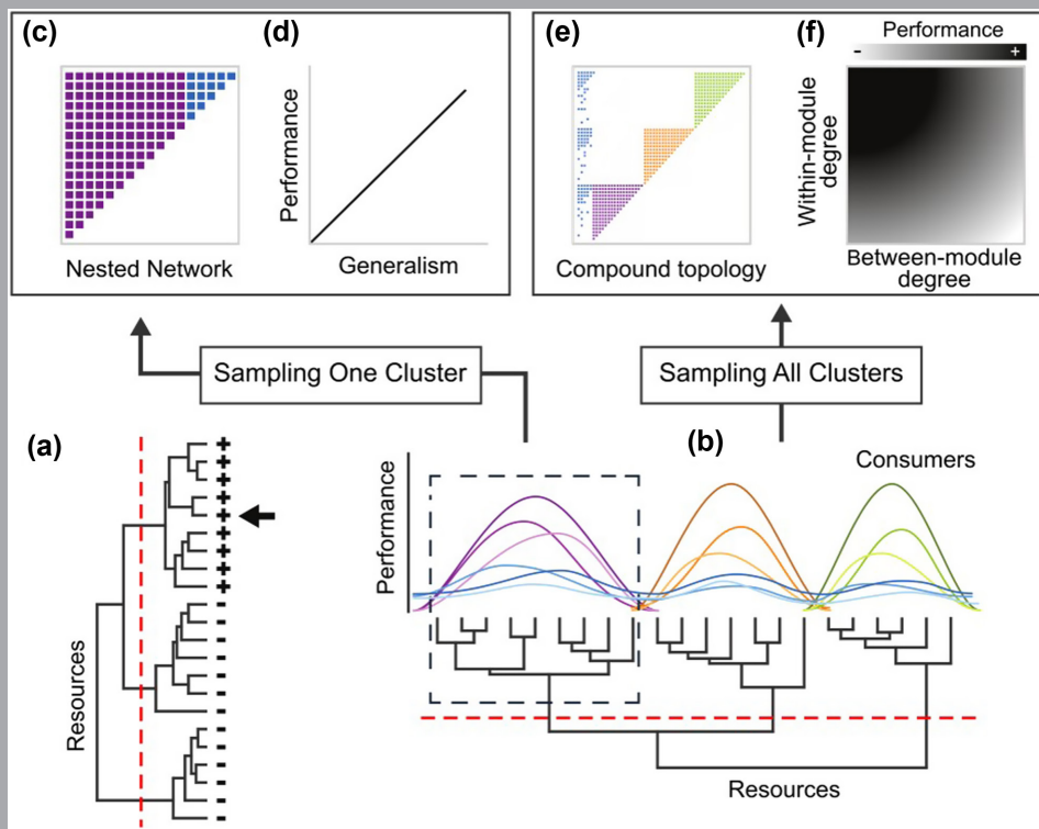
Figure 1. The integrative hypothesis of specialization. (a) If the dissimilarity among resources is represented as a dendrogram, then a mutation that enhances the performance of a consumer in a focal resource (the black arrow), should also represent an adaptation to exploit closely related resources (+), but a maladaptation for distant resources (-). The red dashed line marks the dendrogram level above which dissimilarities among clusters of resources become sufficiently large to turn adaptations for one cluster into maladaptations for other clusters. (b) The expected pattern of consumer performance on resources. On the one hand, only consumers exploiting resources in different clusters (blue) are expected to suffer from tradeoffs in generalism. On the other hand, the performances of consumers specialized in one cluster (purple, orange and green) should be correlated in different resources of that cluster. Then, by sampling consumers exploiting resources of a single cluster, we should find a nested interaction matrix (c) and a positive relationship among performance and generalism (d). Otherwise, by sampling consumers exploiting resources at different clusters, we should find a compound interaction network (e) and a dependence on the signal of the relationship between generalism and performance to the type of generalism analyzed: positive for within-module generalism and negative for between-modules generalism (f).
