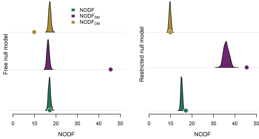
Figure 3. Observed values (dots) of NODF , NODF_{SM} and NODF_{DM} in the regional network contrasted with the values expected by species degrees (distributions) in the absence (free null model) or presence (restricted null model) of a modular structure. NODF : overall nestedness. NODF_{SM} : nestedness between pairs of species of the same module. NODF_{DM} : nestedness between pairs of species of different modules. As expected if the regional network has a compound topology, NODF_{SM} is higher than expected given the modular structure, that is, by the restricted null model.
